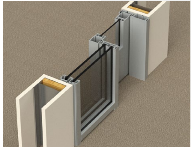
▲ Section Double Glazed Aluminum Sliding Door
