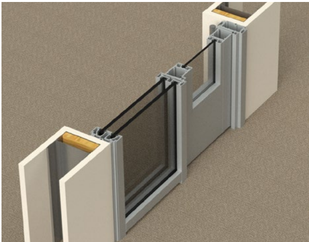
▲ Section Double Glazed Aluminum Swing Door
