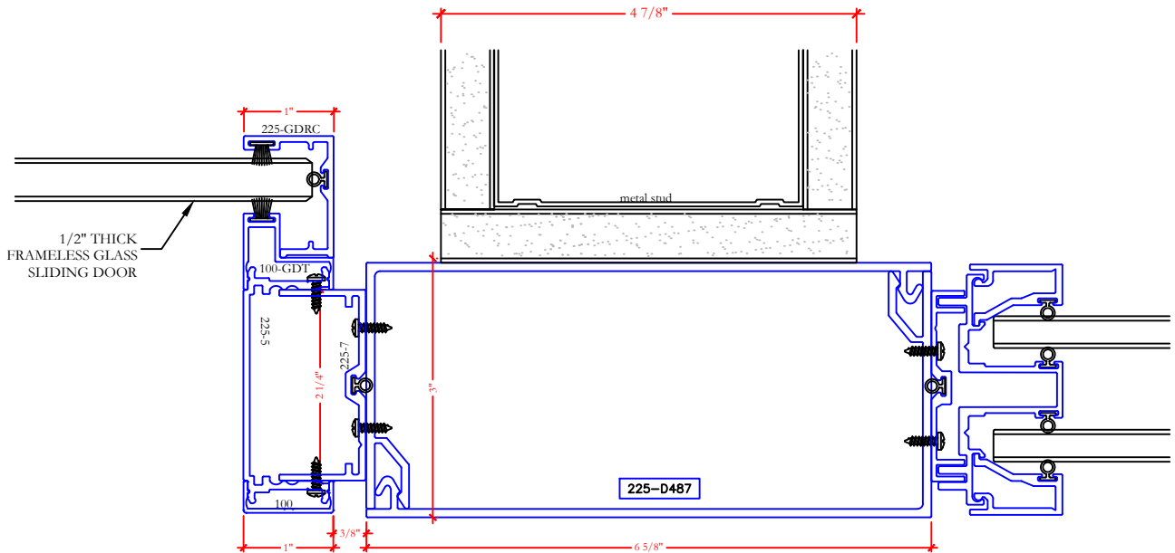
L DEMISING WALL POST (4-7/8" WALL) Scale: Half
