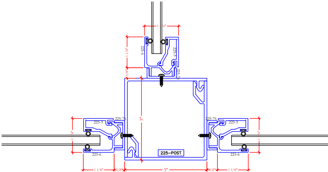
N 3-WAY POST Scale: Half
