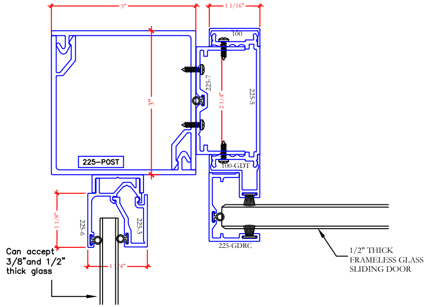
J SLIDING DOOR AT 90 DEGREE CORNER Scale: Half
