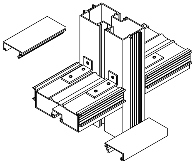
9A HORIZONTAL MUNTIN TO VERTICAL MULLION SC1 CLIPS – 2 REQUIRED EACH
