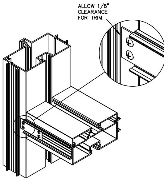
10 HORIZONTAL MUNTIN TO DOOR JAMB FC1 CLIPS – 2 REQUIRED NOTE: ALL TRIM, EXCEPT 1", WILL NEED TO BE NOTCHED AT THIS CLIP (SEE DETAIL 7)
