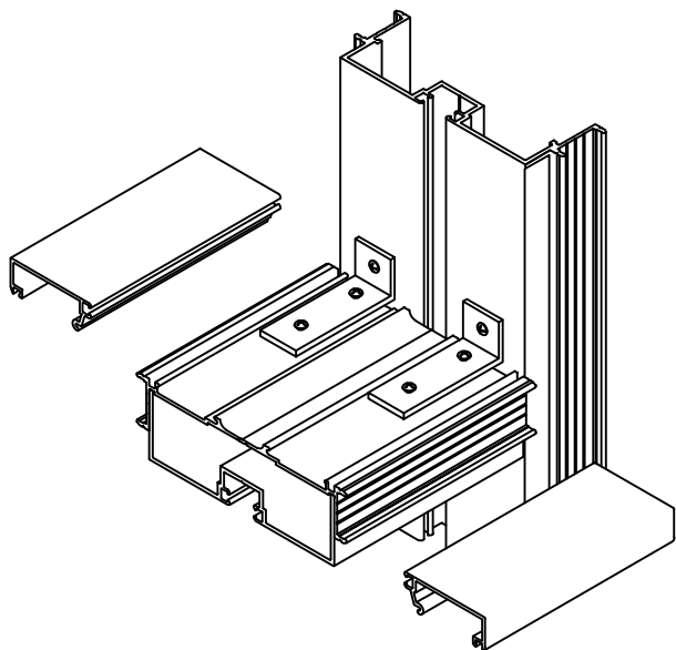
8A HORIZONTAL MUNTIN TO JAMB MULLION SC1 CLIPS – 2 REQUIRED
