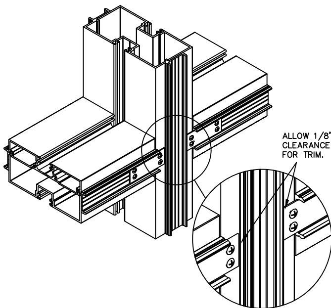
9 HORIZONTAL MUNTIN TO VERTICAL MULLION FC1 CLIPS – 2 REQUIRED EACH NOTE: ALL TRIM, EXCEPT 1", WILL NEED TO BE NOTCHED AT THIS CLIP (SEE DETAIL 7)
