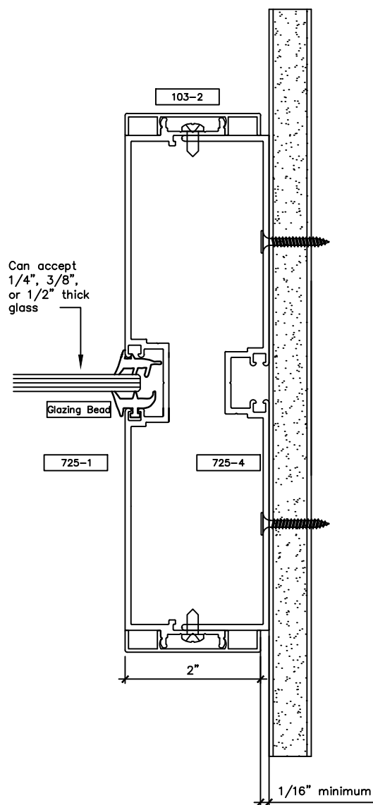
D1 GLASS JAMB WITH WALL STARTER Scale: Half Dwg File: S725T200_03.dwg
