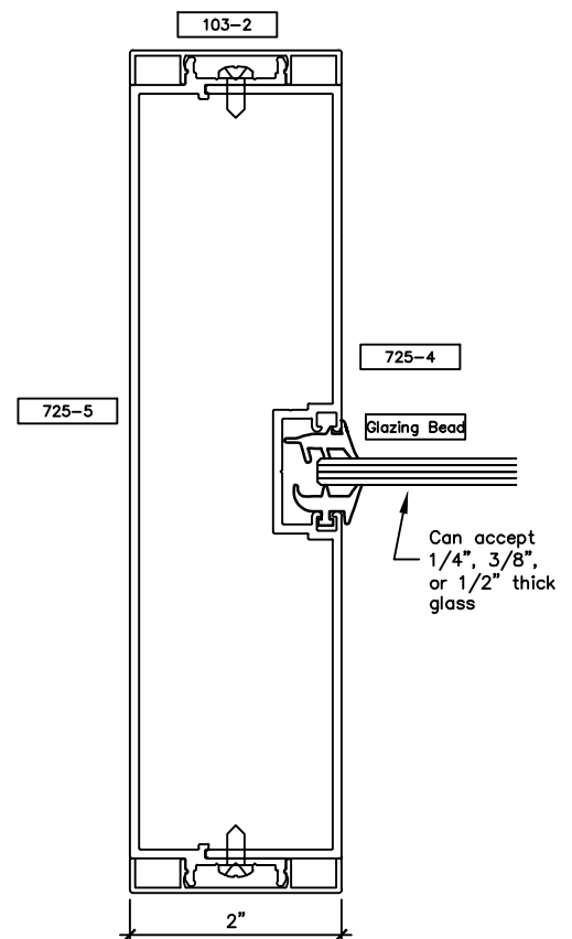
L CASED OPENING JAMB WITH SIDELITE Scale: Half Dwg File: S725T200_08.dwg
